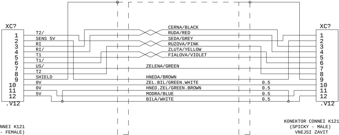
CONNECTOR CONNEI POHLED ZE STRANY PAJENI LOOK FROM SOLDER SIDE
