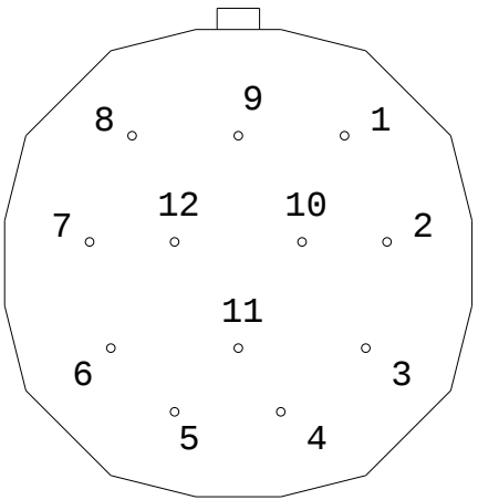
CONNECTOR CONNEI POHLED ZE STRANY PAJENI LOOK FROM SOLDER SIDE
