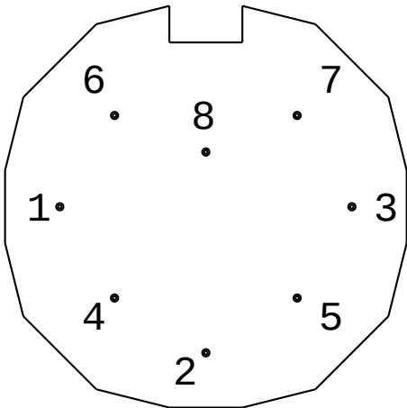
CONNECTOR BINDER POHLED ZE STRANY PAJENI LOOK FROM SOLDER SIDE
