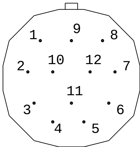
CONNECTOR CONNEI
